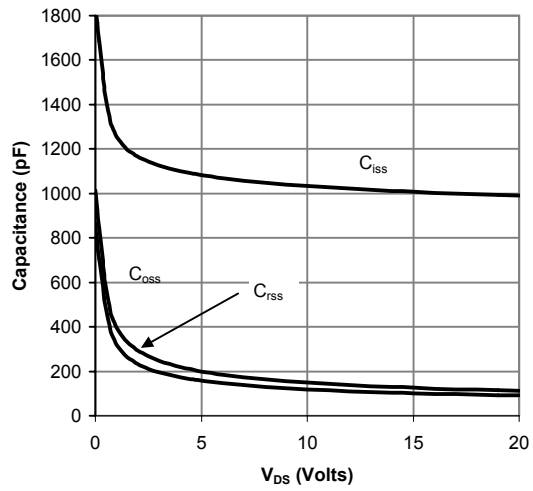
Figure 8: Capacitance Characteristics
