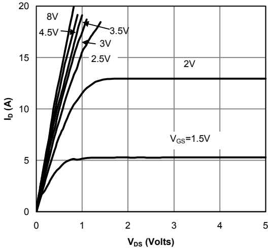
Fig 1: On-Region Characteristics
